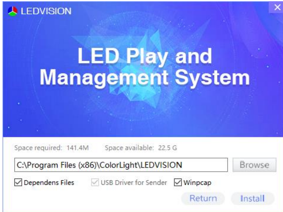
Fig. 2-4 Choose Components
