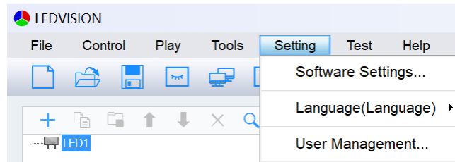
Fig. 3-7 Setting Menu
