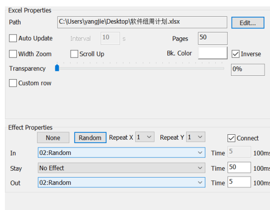
Fig. 5-10 Excel Properties
