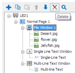
Fig. 4-11 Delete Window
