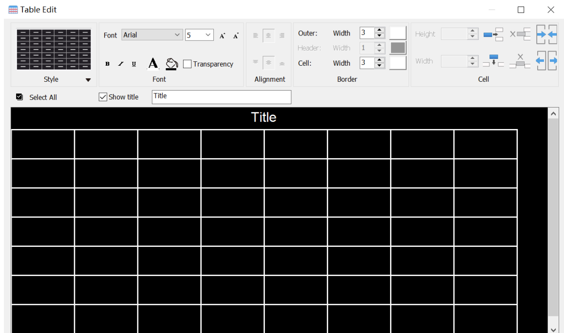
Fig. 5-29 Table Editor
