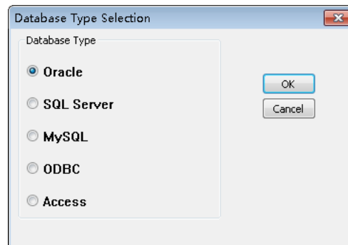
Fig. 5-31 Database Type
