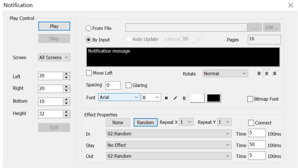
Fig. 6-1 Notification Management
