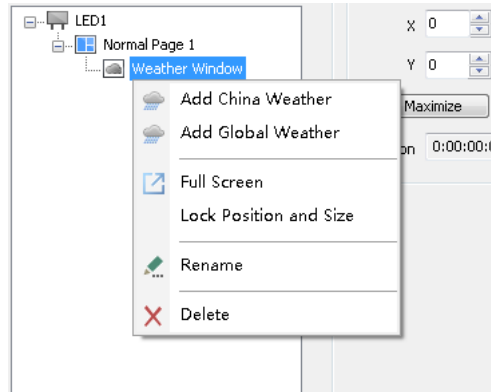
Fig. 5-43 Weather Type
