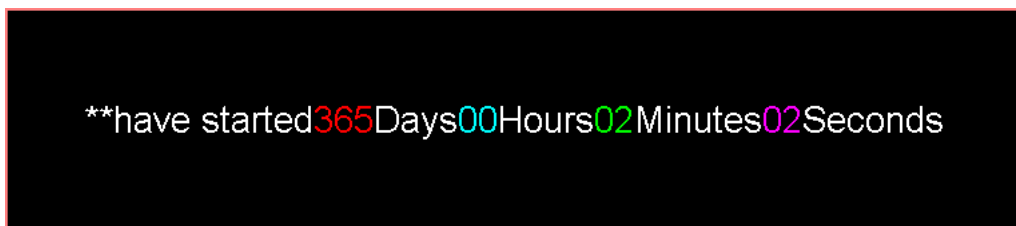
Fig. 5-24 Timer Effect
