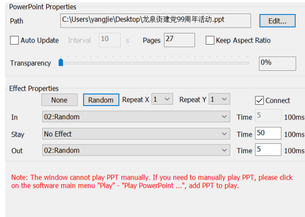
Fig. 5-11 PowerPoint Properties
