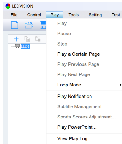
Fig. 3-5 Play Menu
