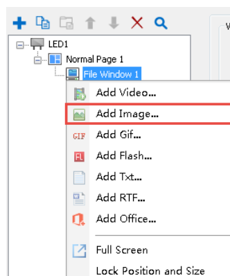
Fig. 5-3 Add Image
