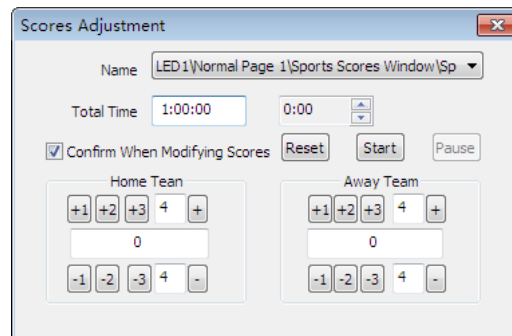
Fig. 5-58 Score Adjustment
