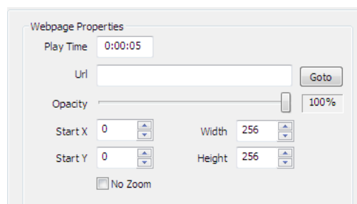
Fig. 5-27 Webpage Zoom
