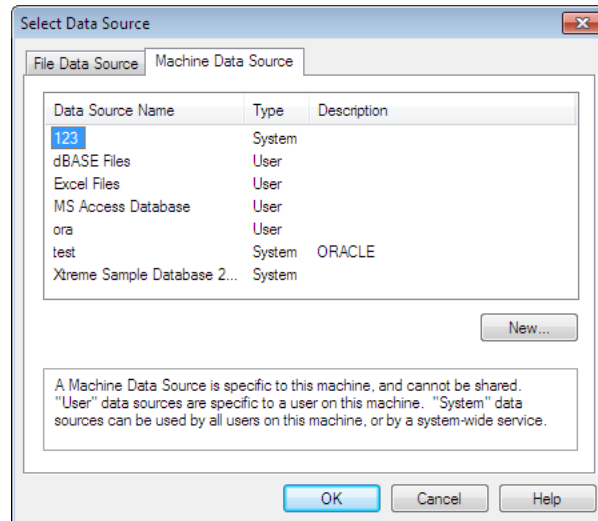
Fig. 5-36 ODBC Setting
