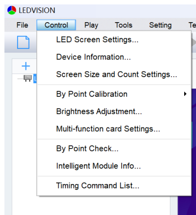
Fig. 3-4 Control Menu
