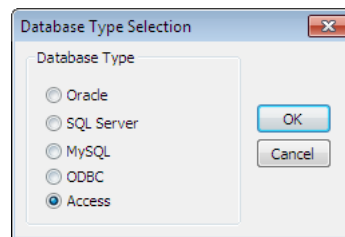
Fig. 5-39 Select Access
