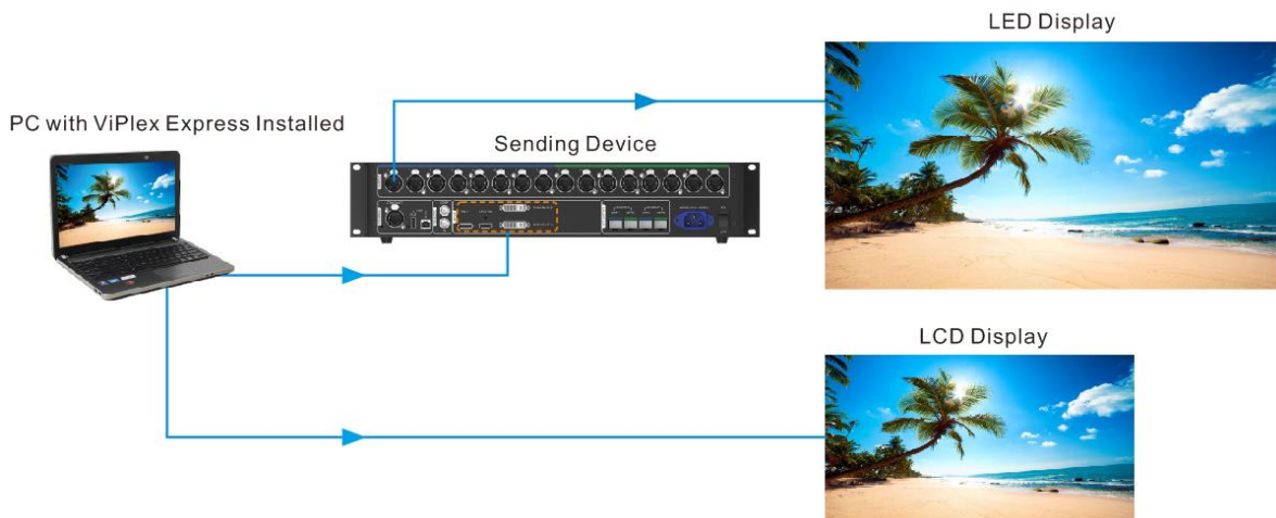
Figure 2-8 Connecting to displays
