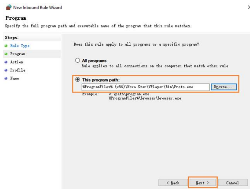
Figure 7-4 Program selection
