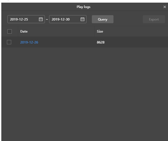
Figure 5-2 Query result
