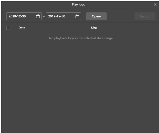
Figure 5-1 Play logs
